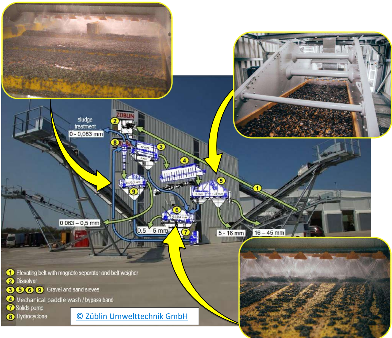
Figure 3: Treatment steps of the soil washing plant.
