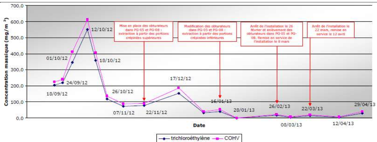
Evolution of the mass content of trichloroethylene in the air flow extracted from the ground
