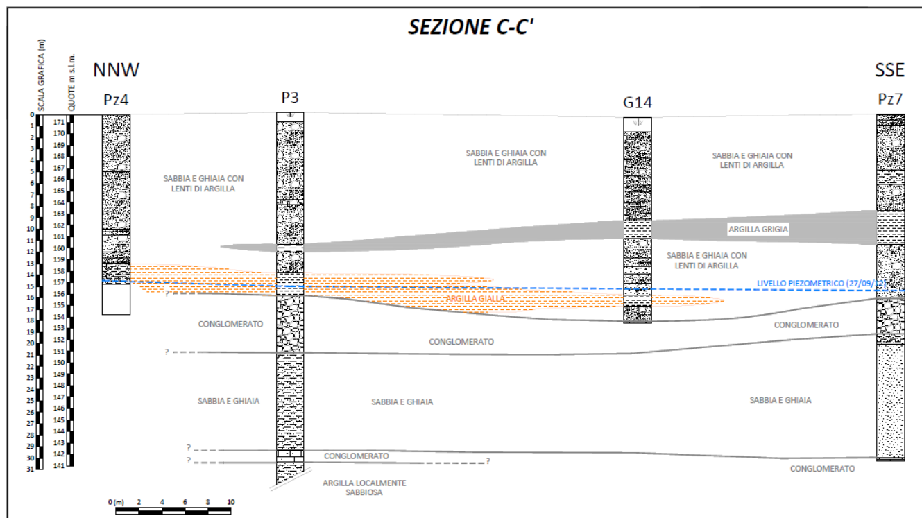
Stratigraphic detail of the intervention area
