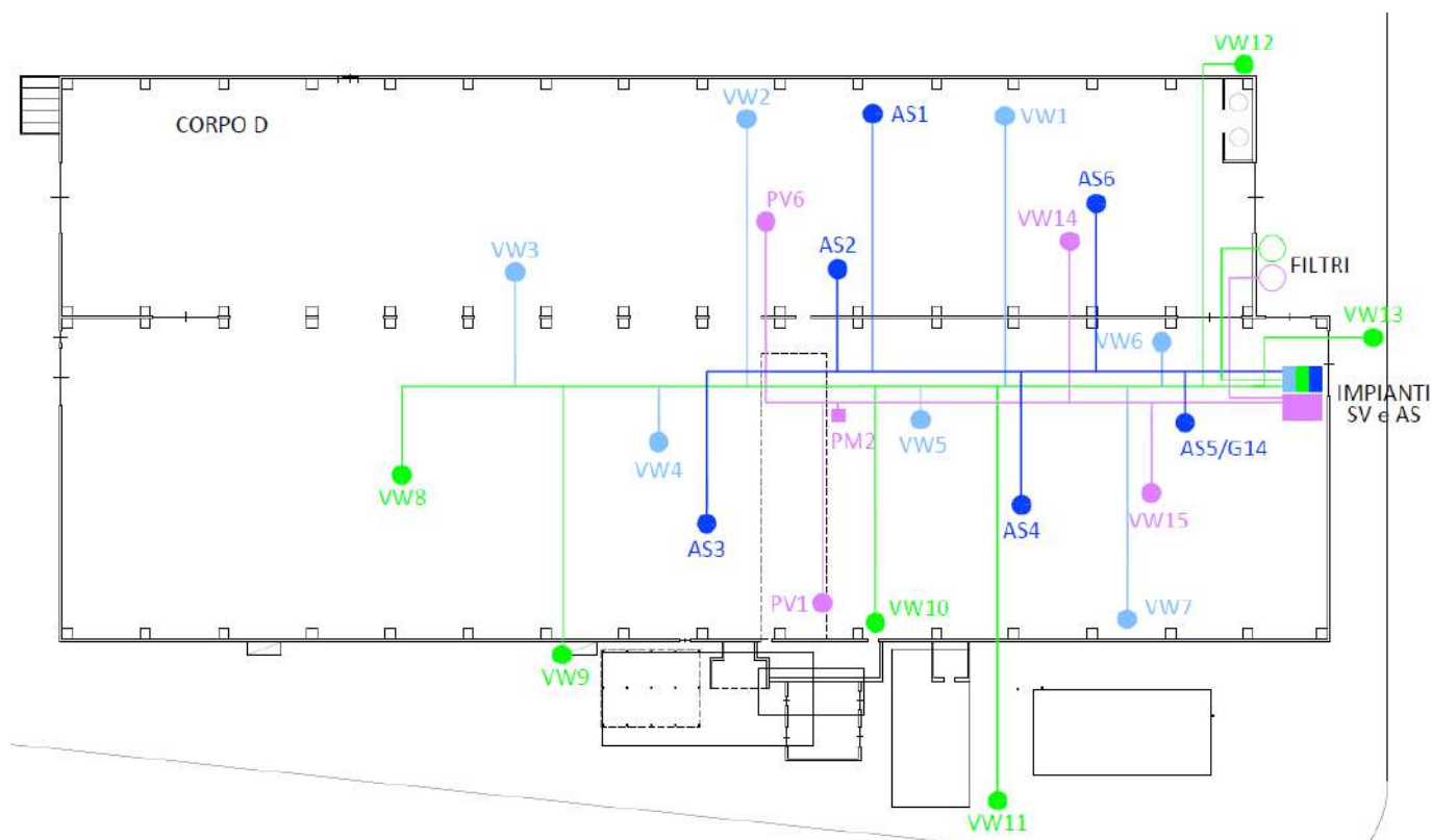
Position of the AS and SVE wells
