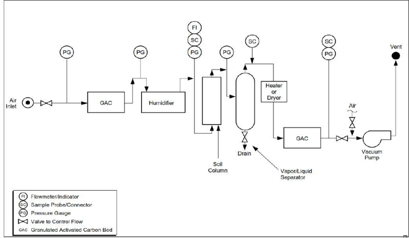
Figure 3.3- Diagram of a column test apparatus
