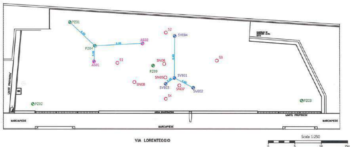
Figure 4.5- Typical positioning at 120° of SVE monitoring point (Confalonieri et al., see Annex1)
