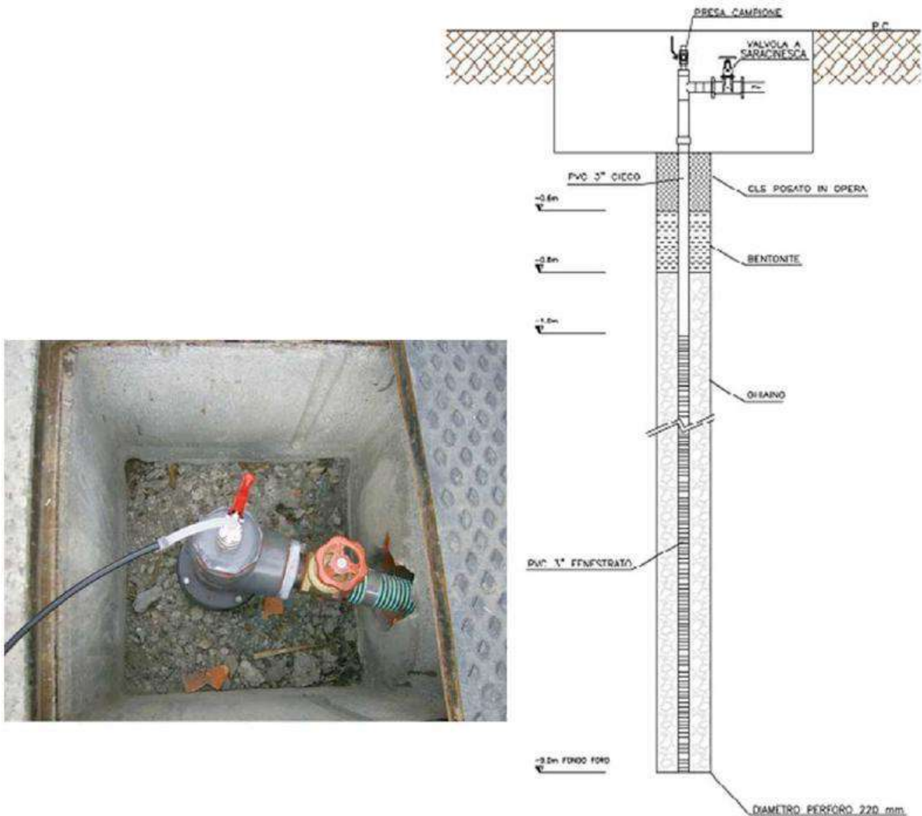
Figure 4.8- Example of Nesty Probe installation (Trezzani et al., see Annex1)
