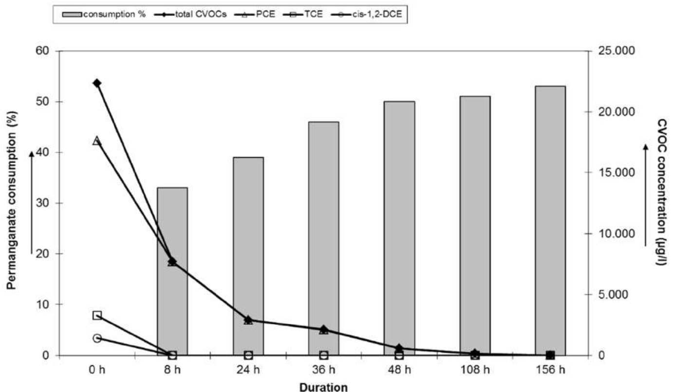
Laboratory test, oxidation of CVOC contaminated groundwater from monitoring point GWM 3423 using permanganate
