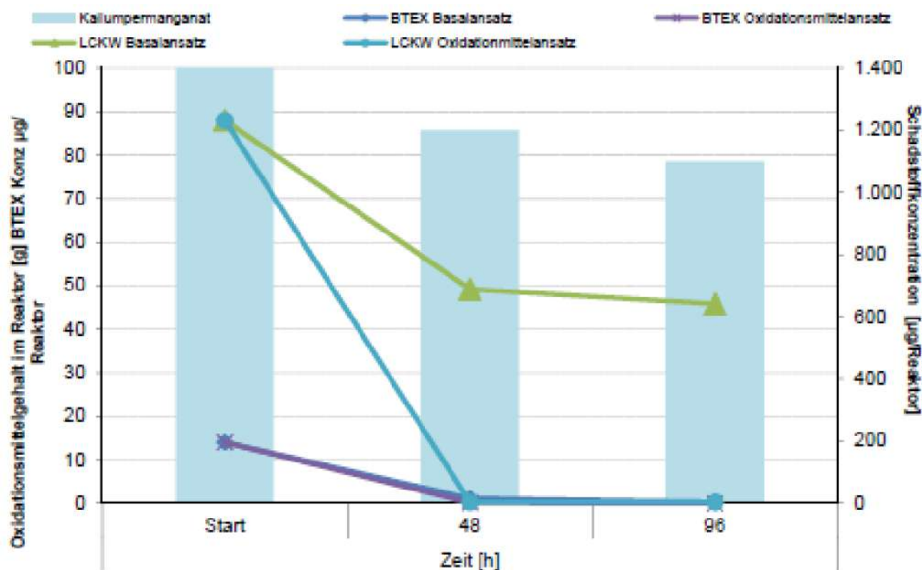
Oxidant consumption (KMnO 4 ) and contaminant reduction (CHC and BTEX) during 96 hr reactor test
