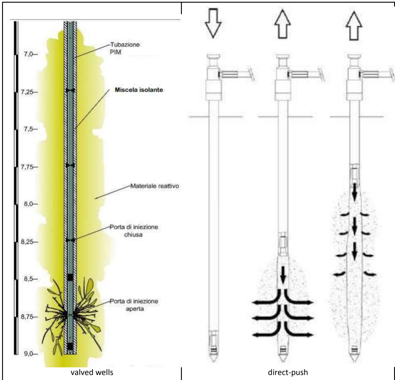
Figura 4.2 – Pozzi a valvola e Direct-push ( https://www.carsico.it/servizi/ )
