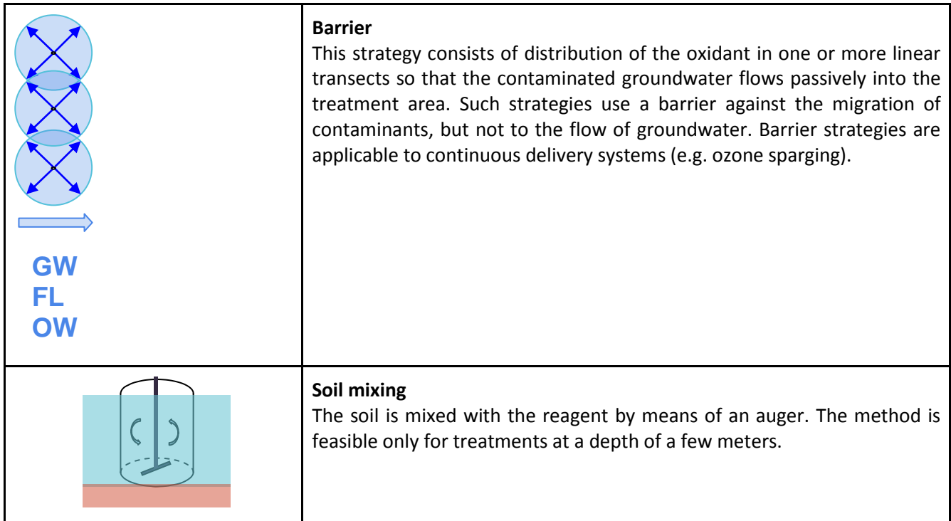
Figure 4.3- Types of injection strategies
