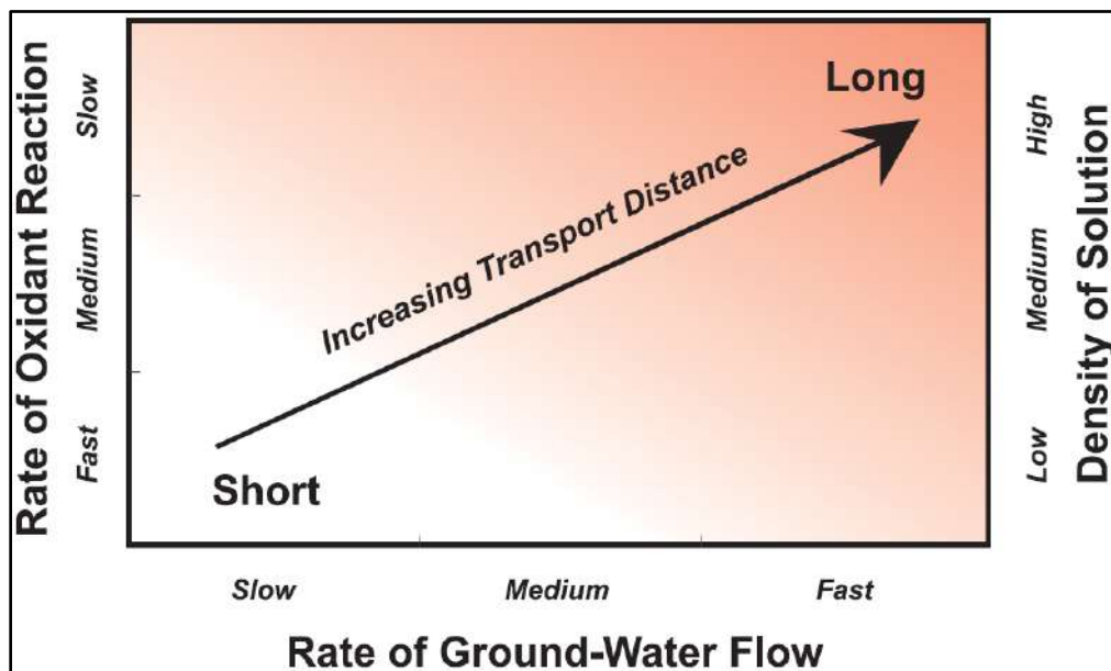
Figure 4.1 – rate of oxidant reaction/density of solution, as a function of rate of groundwater flow
