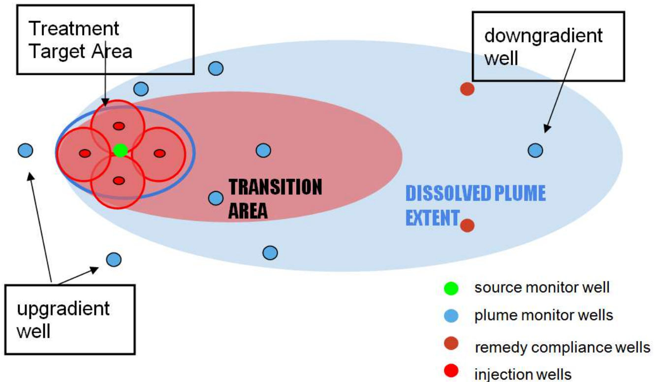
Figure 4.4: Position of the monitoring wells
