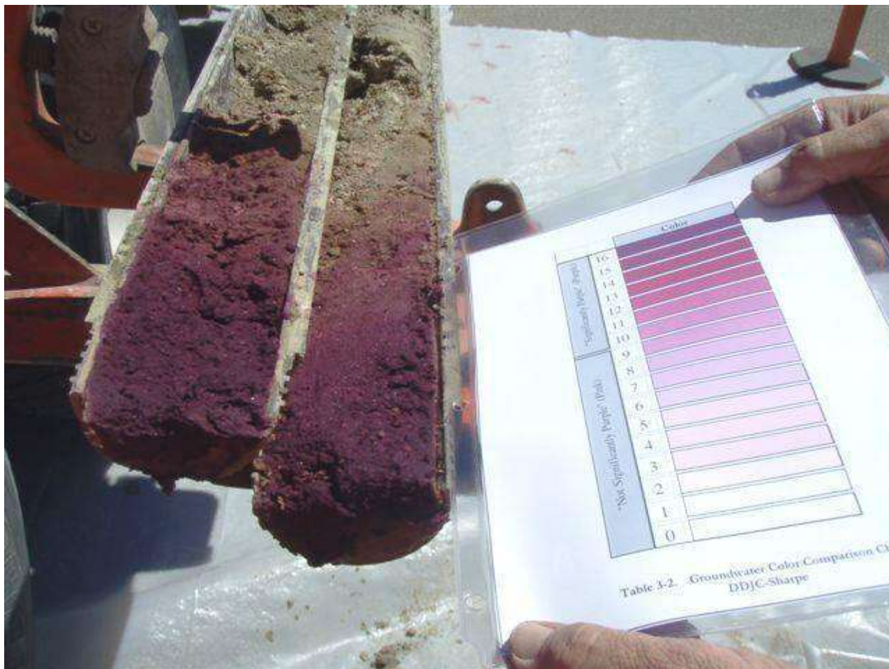
Figure 2.8- Example of oxidant diffusion profiling in silt soil cores 90 days after fracture-emplacment of potassium permanganate oxidant slurry (photo courtesy of URS, Bures archive)
