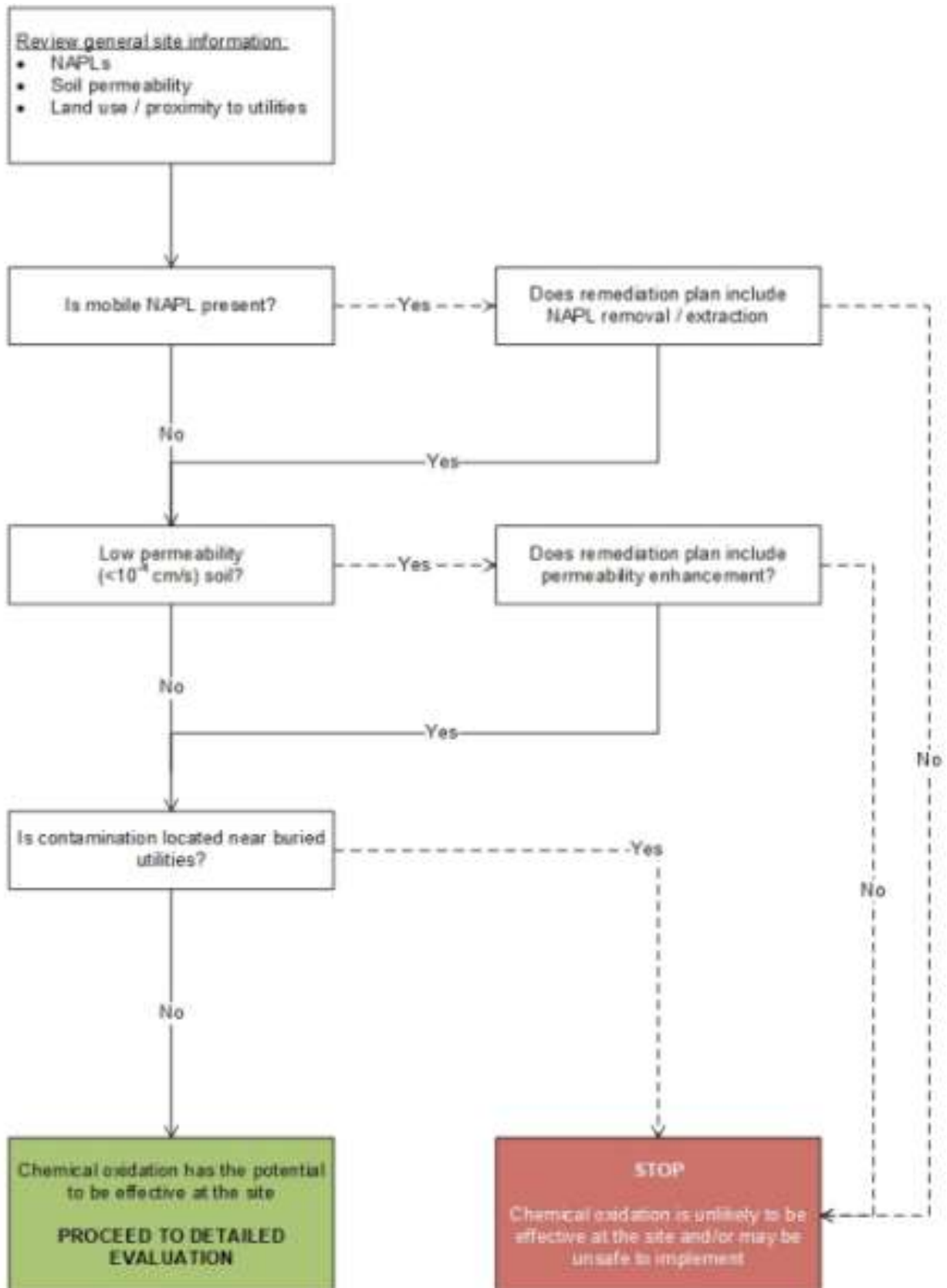
Figure 3.1- Initial screening for potential effectiveness of ISCO, from US EPA (2004)
