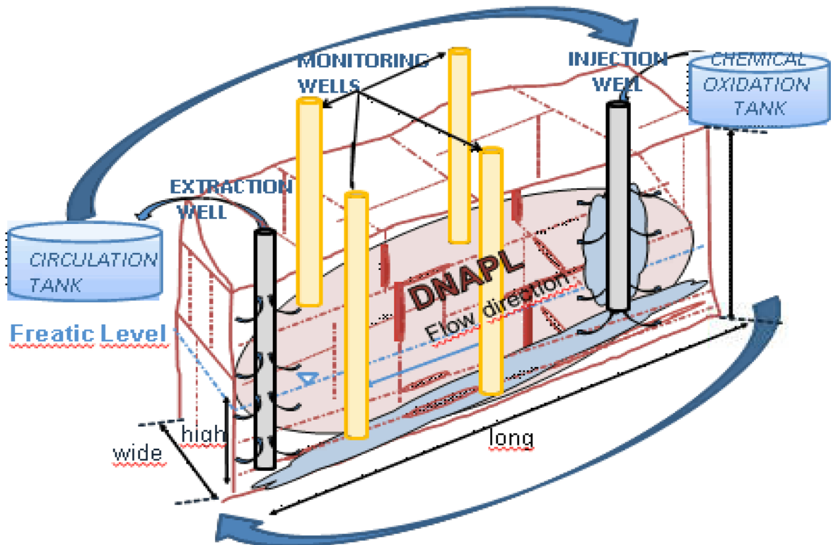
Figure 2.4- 3D Scheme recirculation system
