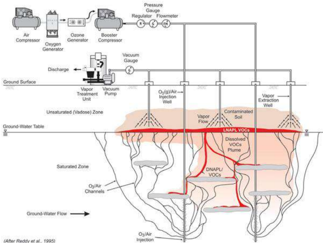
Figure 2.9- General conceptual model of in-situ ozonation in the saturated zone with soil vacuum extraction to capture volatile emissions and O 3 .
