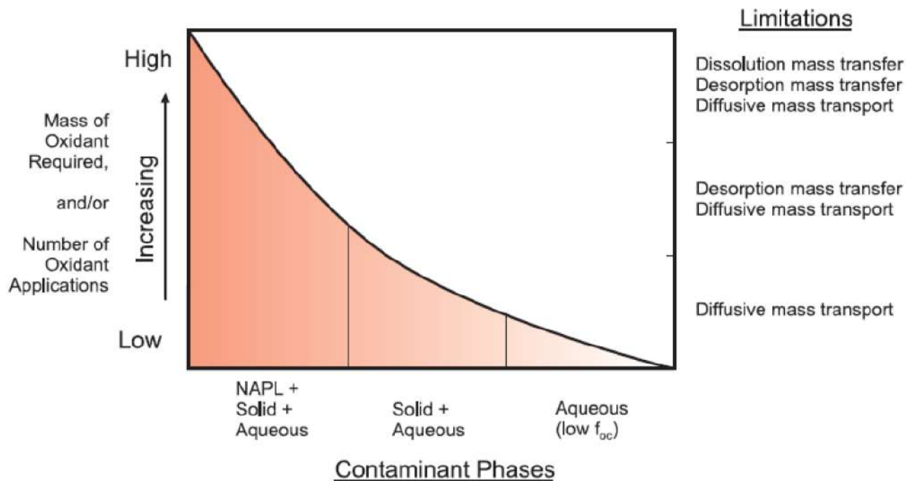
Figure 3.2- Impact of contaminant phases, mass transfer, and mass transport limitations on the mass of oxidant and/or the number of oxidant applications needed for ISCO
